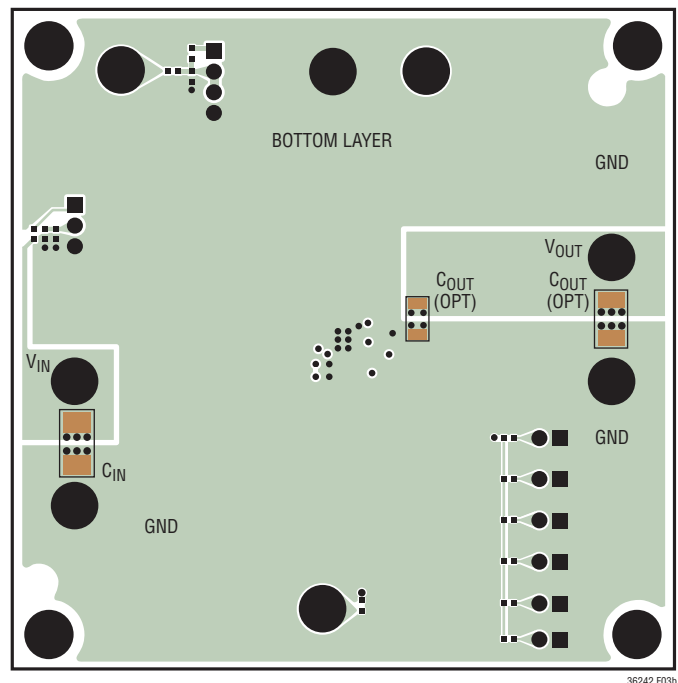
Figure 3b. Sample PCB Layout-Bottom Side
