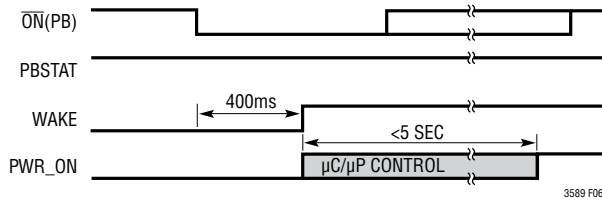
Figure 6. Power-Up Using the Pushbutton
