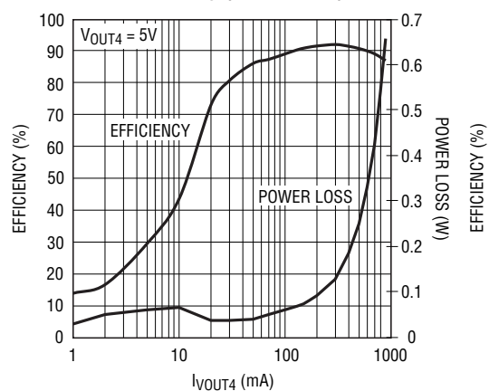
Boost Efficiency ( V_{IN4} = 3.8\text{V} )
