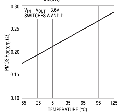
PMOS R_{DS(ON)}
