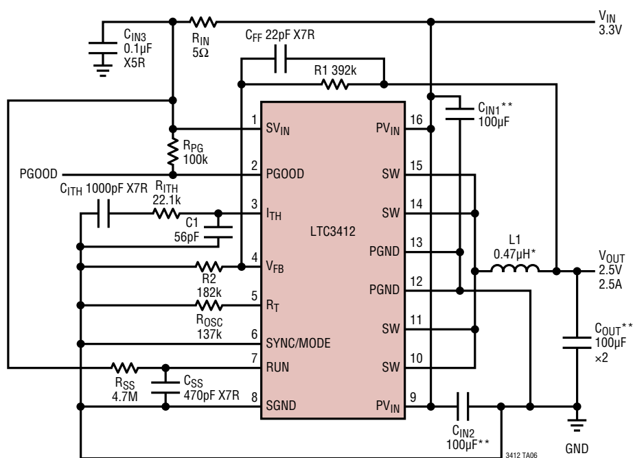
2.5V, 2.5A Low Output Noise Regulator at 2MHz
