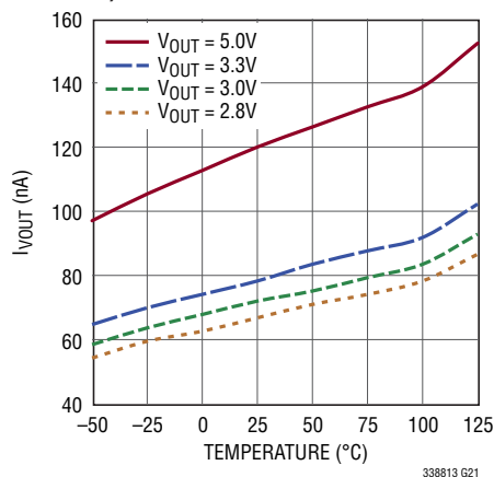
I VOUT vs Temperature (LTC3388-3)
