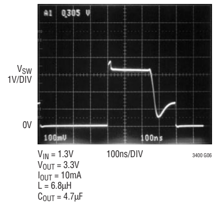
SW Pin Antiringing Operation
