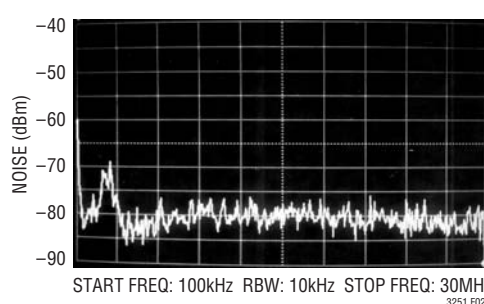
Figure 2b. LTC3251 Output Noise Spectrum with 10µF Output Capacitor ( I_O = 500\text{mA} )
