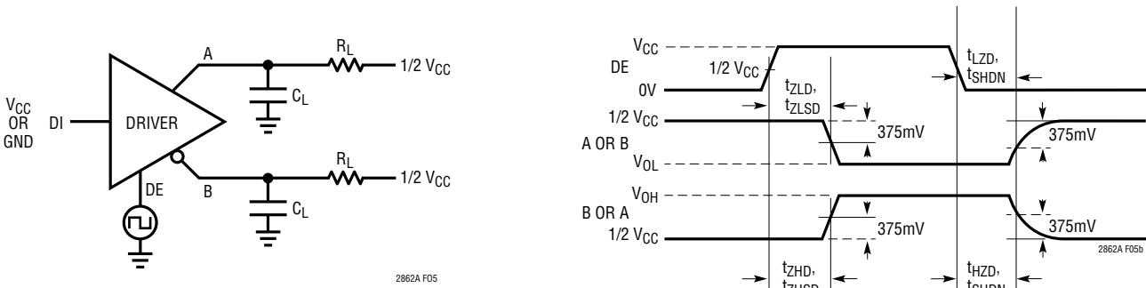
Figure 5. Driver Enable and Disable Timing Measurements
