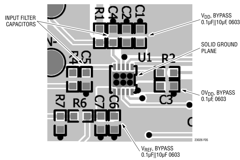
Figure 5. Suggested Layout
