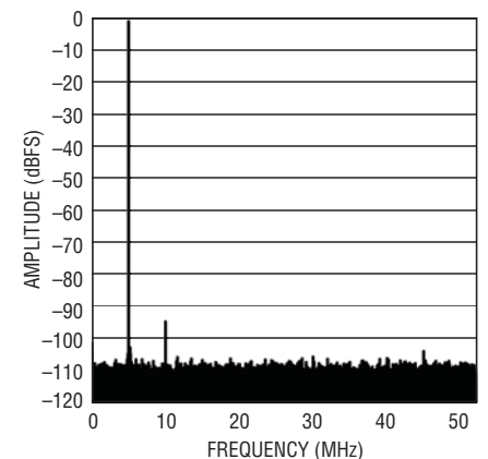
LTC2144-12: 64k Point FFT, f_{IN} = 5\text{MHz} , -1dBFS, 105Msps
