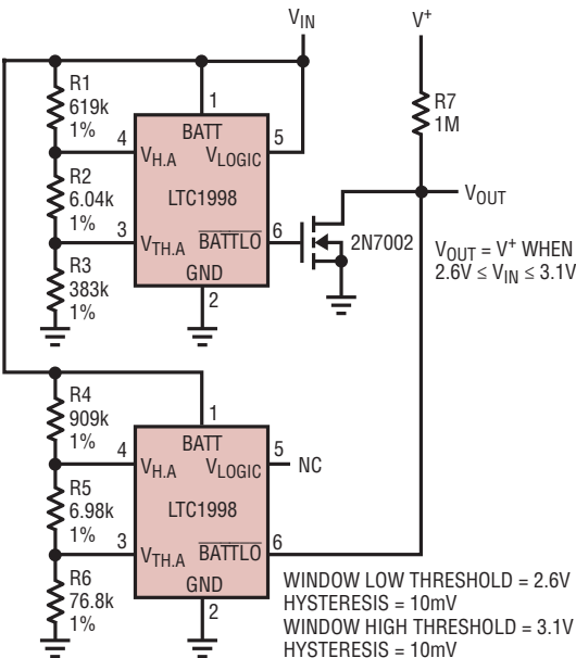
High Accuracy Window Comparator with Dual Hysteresis
