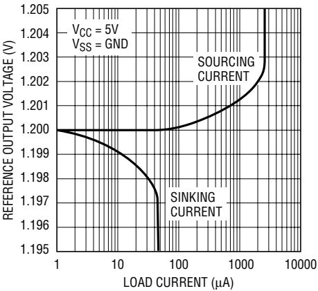
Reference Output Voltage vs Load Current
