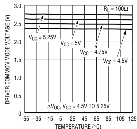
Driver Common Mode Output Voltage vs Temperature
