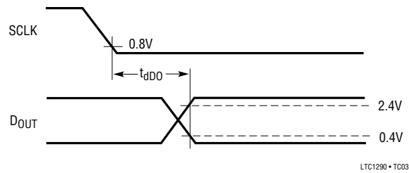
Voltage Waveforms for D_{OUT} Delay Time, t_{dDO}
