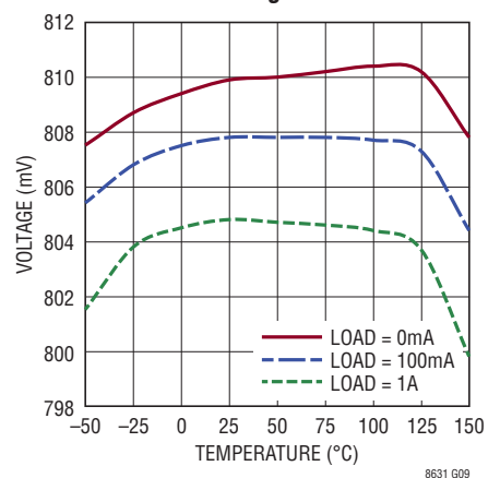
Reference Voltage
