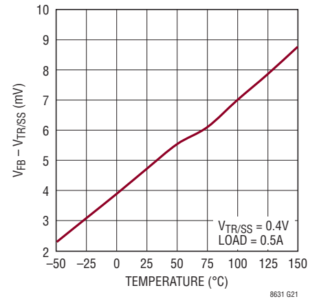
FB to TR/SS Offset Voltage
