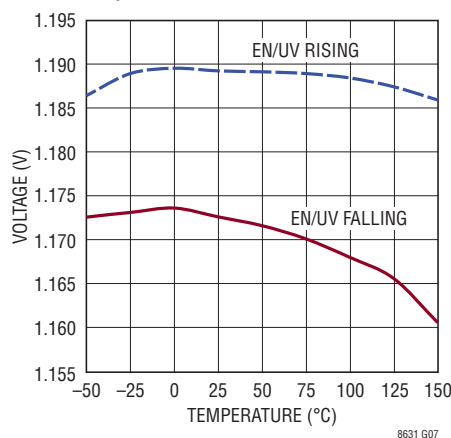
EN/UV Thresholds
