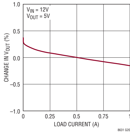
Load Regulation
