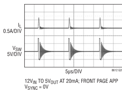
Switching Waveforms
