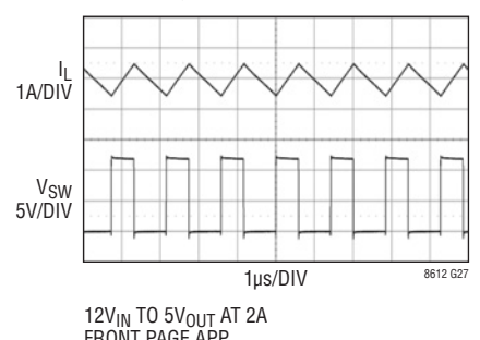
Switching Waveforms
