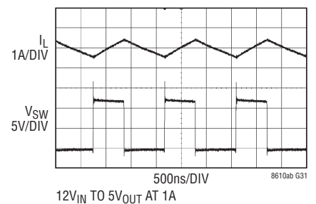
Switching Waveforms
