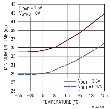
Minimum On-Time
