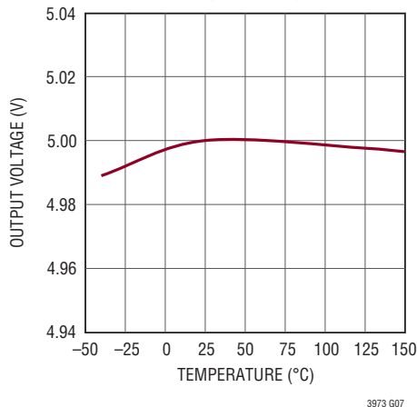
LT3973-5 Output Voltage
