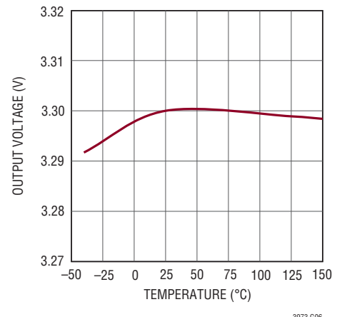
LT3973-3.3 Output Voltage
