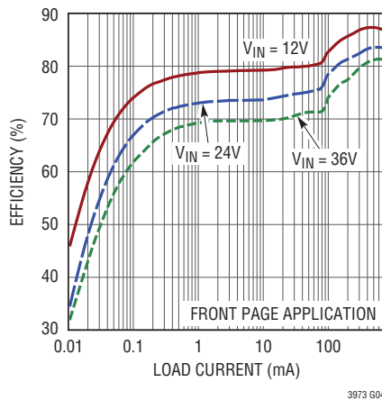
Efficiency, V_{OUT} = 5\text{V}
