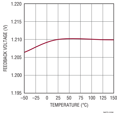
LT3973 Feedback Voltage
