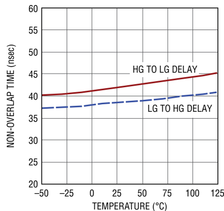
BG and TG Non-Overlap Time
