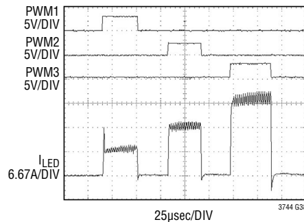
LED Current Waveforms (0A to 6.7A to 13.3A to 20A) 5000:1
