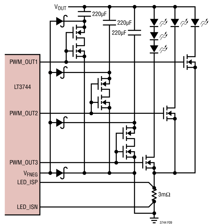
Figure 9. Driving Multiple LEDs from the Same Output Using Schottky Diodes For V_{FNEG}
