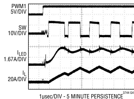
LED Current Waveforms (5000:1) 0A TO 20A Flicker-Free Performance
