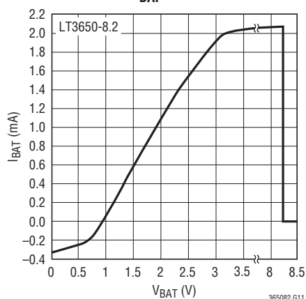
CC/CV Charging; BAT Pin Bias Current vs V_{BAT}
