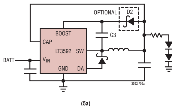
Figure 5. Two Circuits for Generating the Boost Voltage
