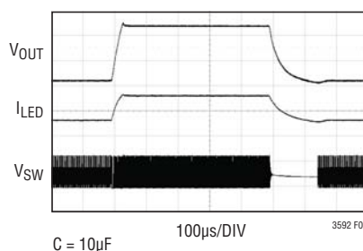
Figure 4. Transient Load Response of the LT3592 with Different Output Capacitors
