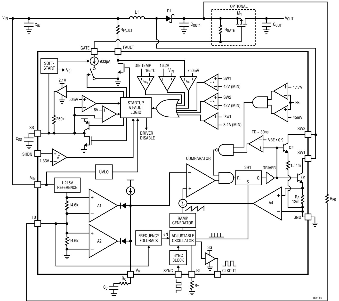
Figure 1. Block Diagram
