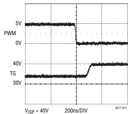
PMOS Turn-Off
