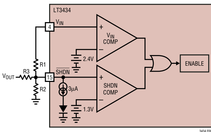
Figure 8. Undervoltage Lockout
