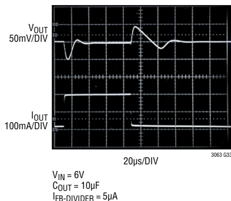
5V Transient Response C_{FF} = 10\text{nF} , I_{OUT} = 20\text{mA} to 200\text{mA}
