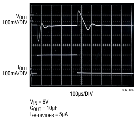
5V Transient Response C_{FF} = 0 , I_{OUT} = 20\text{mA} to 200\text{mA}
