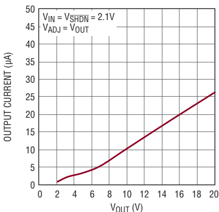
Reverse Current
