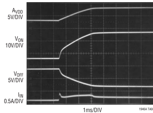
Start-Up Waveforms
