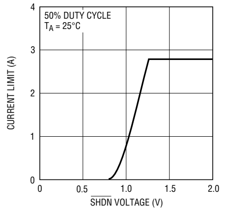
Peak Switch Current vs \overline{SHDN} Pin Voltage (Soft-Start)
