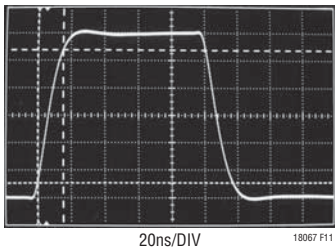
Figure 11. Step Response with R_F = 499k
