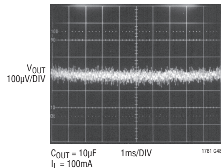
LT1761-5 10Hz to 100kHz Output Noise C_{BYP} = 0.01µF
