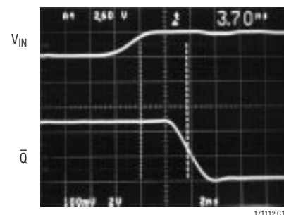
Output Falling Edge, 5V Supply
