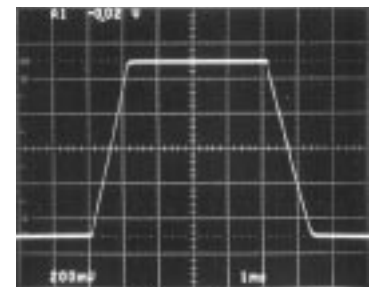
Large-Signal Response V_S = 5V, 0V
