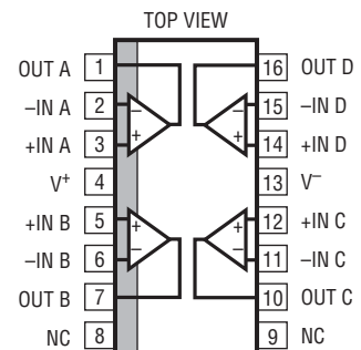
GN PACKAGE 16-LEAD PLASTIC SSOP T_{JMAX} = 150^\circ\text{C} , \theta_{JA} = 135^\circ\text{C/W}
