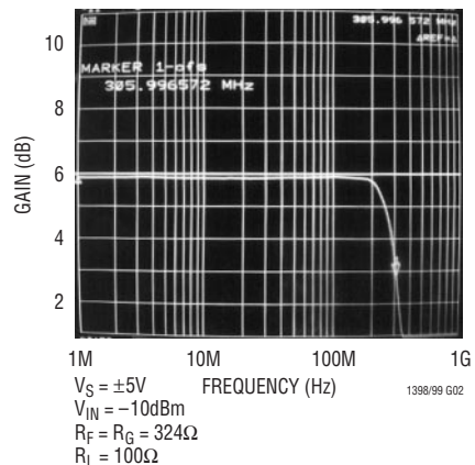
Closed-Loop Gain vs Frequency ( A_V = 2 )
