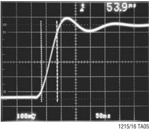
TRANSIENT RESPONSE
