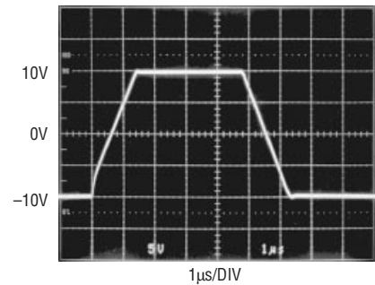
\pm 15V Large-Signal Response
