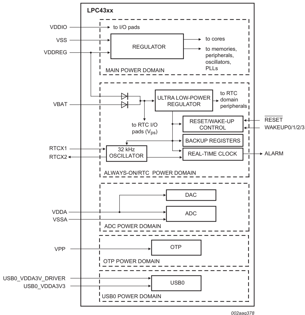
Fig 9. Power domains
