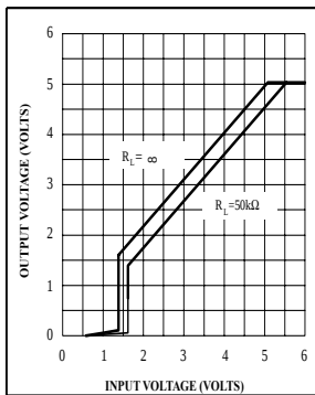
Dropout Characteristics
