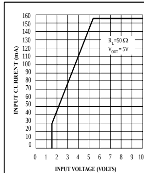
Input Current
