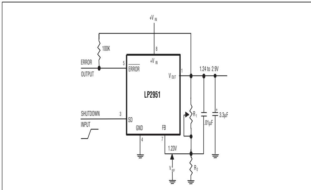
Figure 2. Adjustable Regulator
