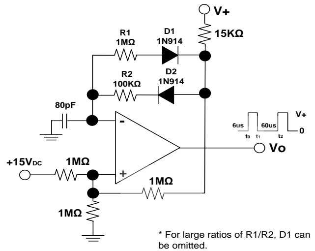
Pulse Generator
