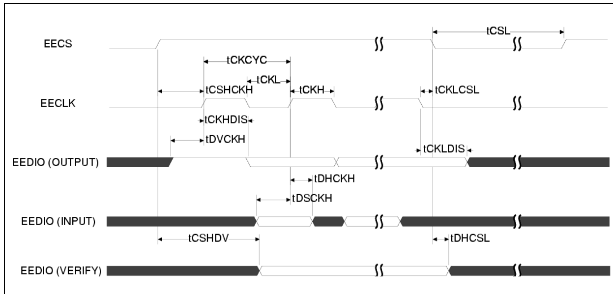
FIGURE 6-10: EEPROM TIMING
