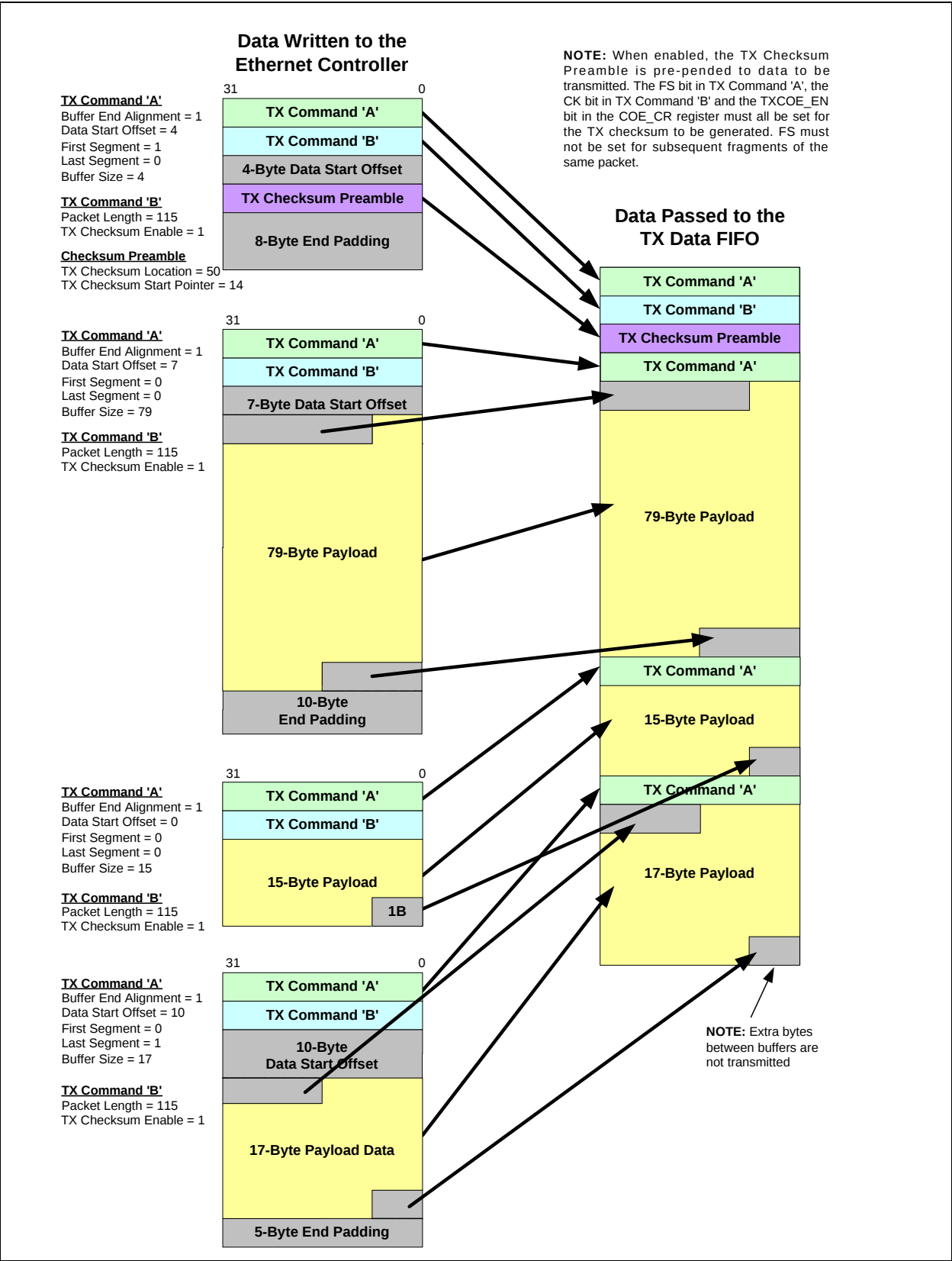
FIGURE 3-23: TX EXAMPLE 3
