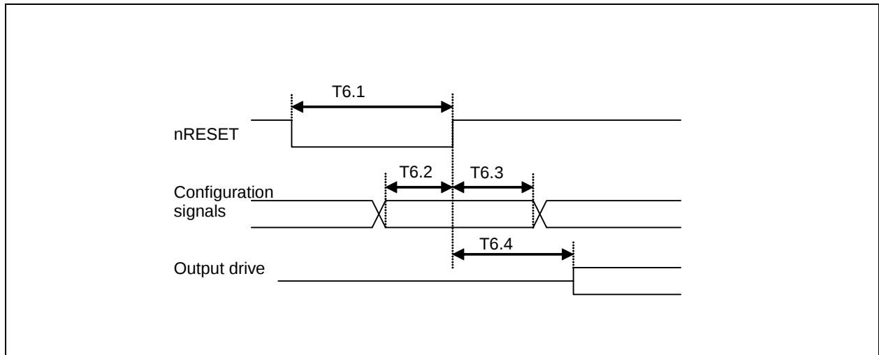
FIGURE 6-9: RESET TIMING
