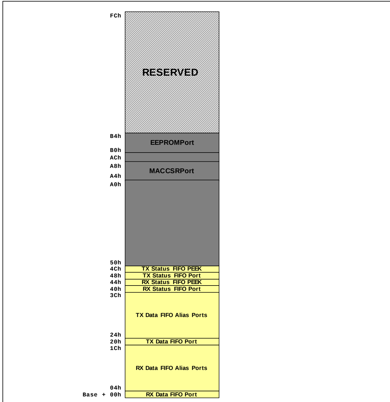
FIGURE 5-1: MEMORY MAP
