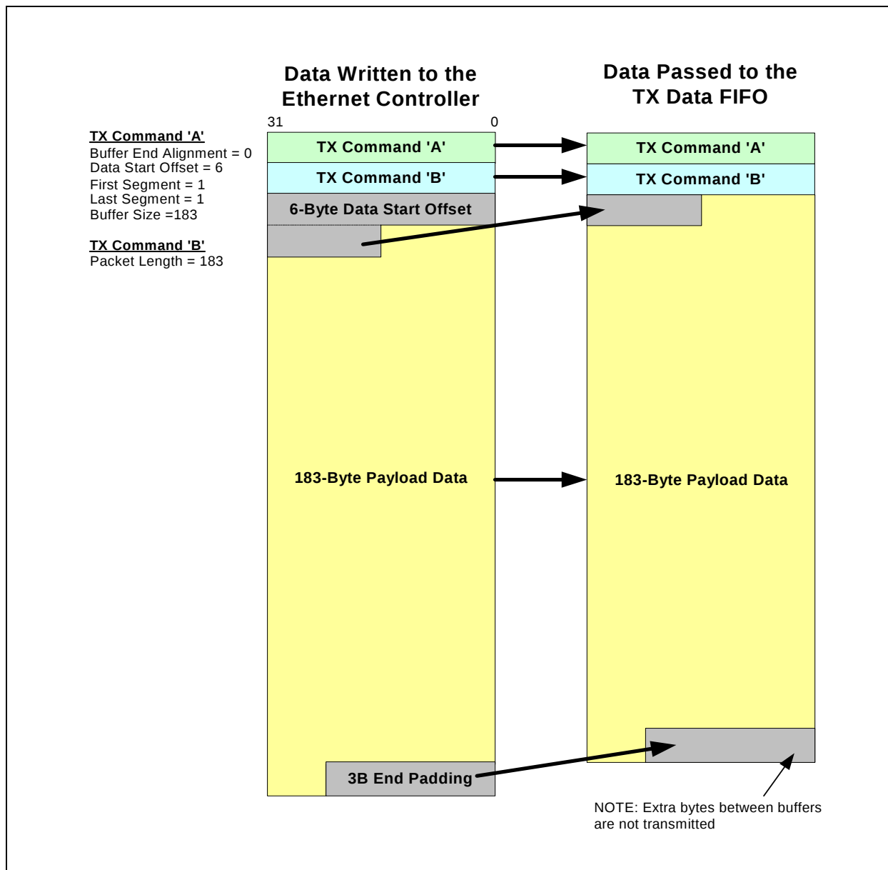
FIGURE 3-22: TX EXAMPLE 2
