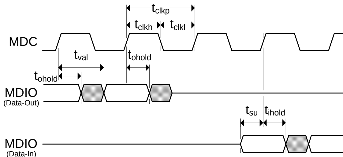
Figure 5.7 SMI Timing
