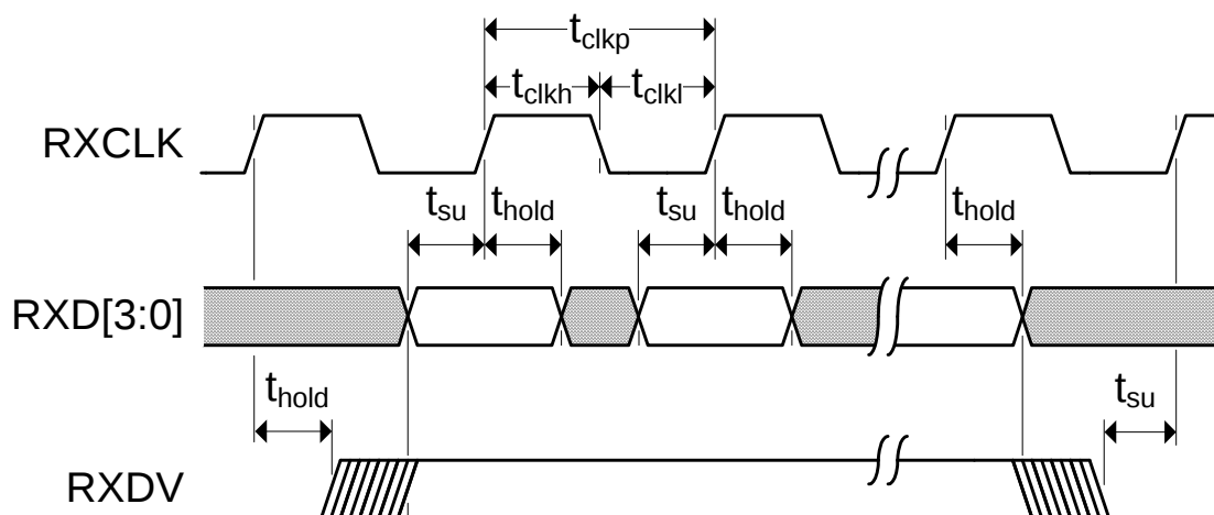
Figure 5.5 MII Receive Timing
