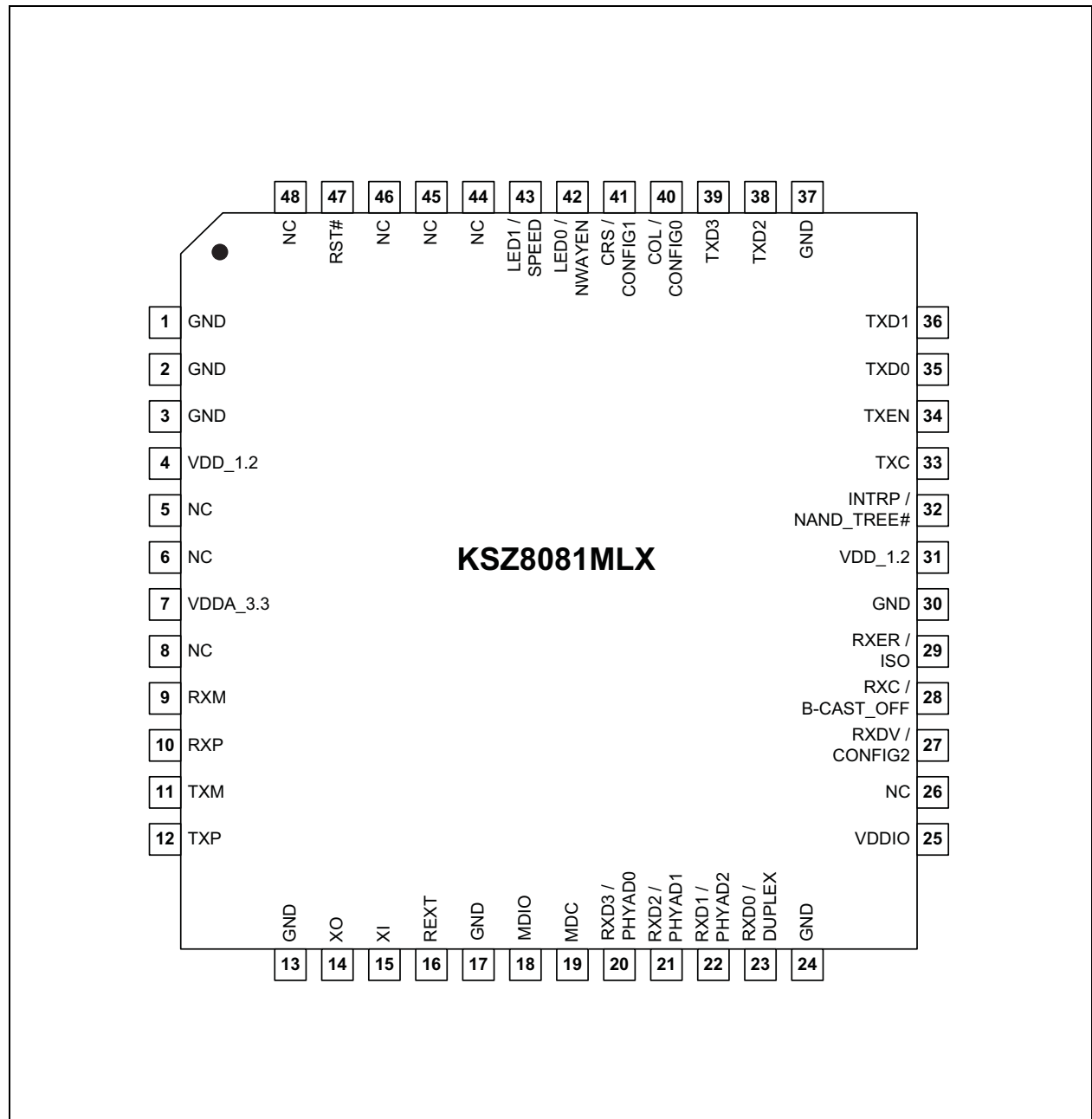
FIGURE 2-1: 48-PIN 7 MM X 7 MM LQFP ASSIGNMENT (TOP VIEW)
