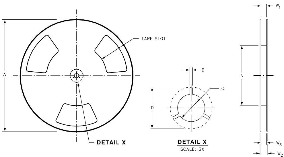
MicroPak 10 Reel Dimensions inches (millimeters)
