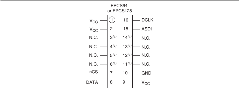
Figure 22. Altera EPCS Device 16-Pin SOIC Package Pin-Out Diagram
