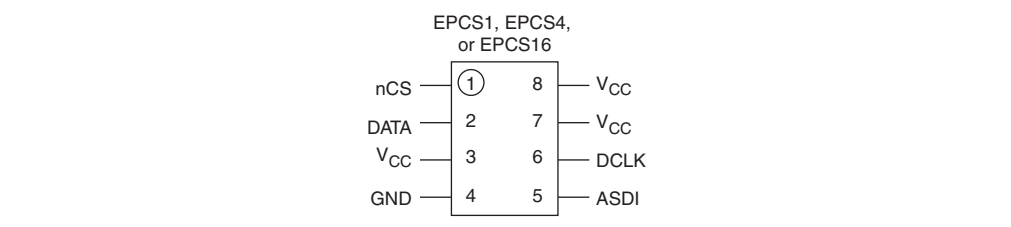
Figure 21. Altera EPCS Device 8-Pin SOIC Package Pin-Out Diagram
