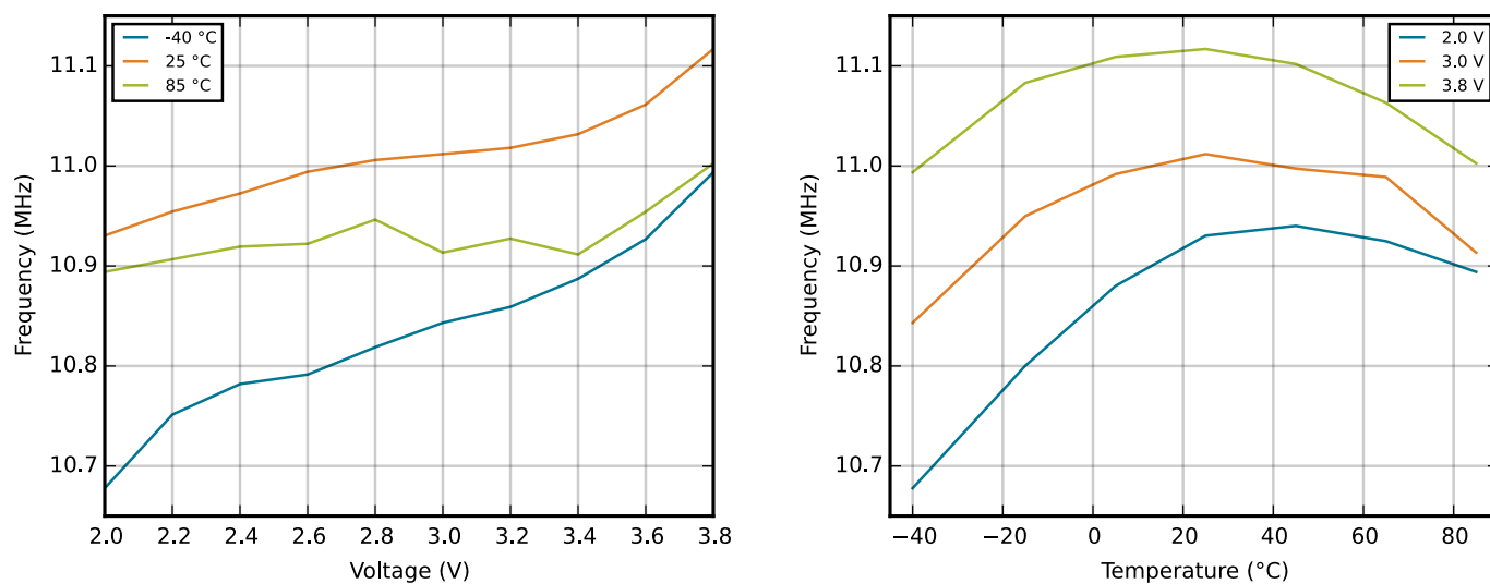
Figure 4.23. Calibrated HFRCO 11 MHz Band Frequency vs Supply Voltage and Temperature
