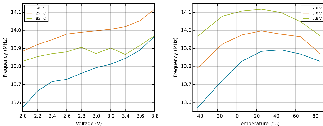
Figure 4.24. Calibrated HFRCO 14 MHz Band Frequency vs Supply Voltage and Temperature
