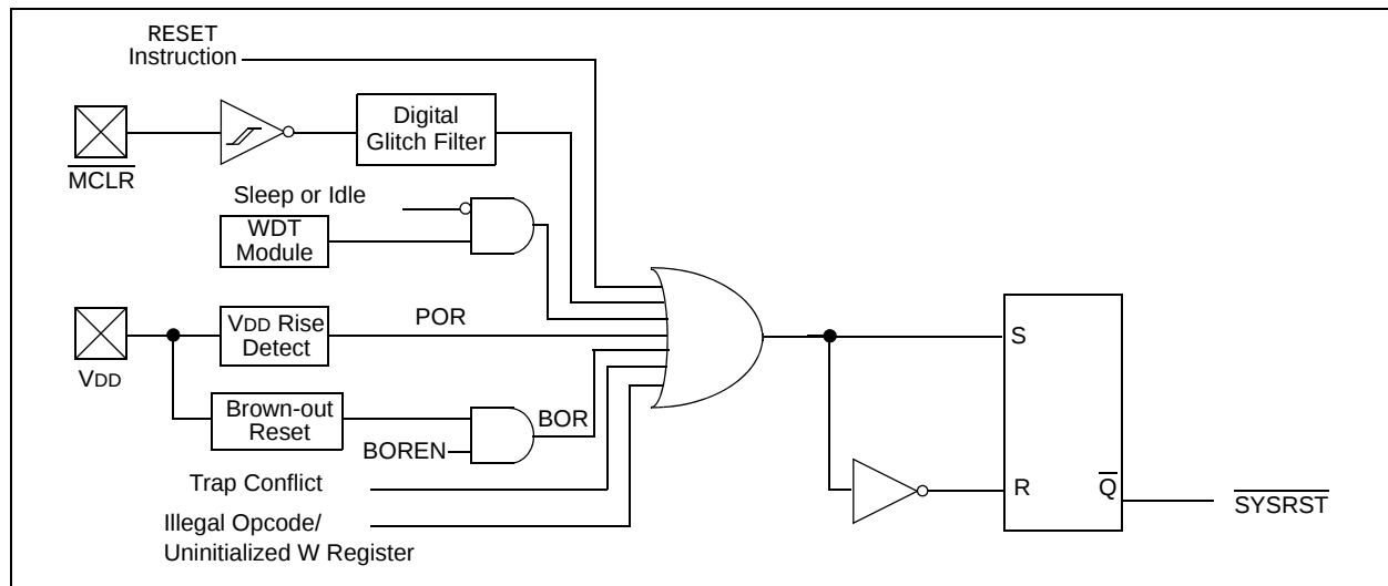
FIGURE 21-2: RESET SYSTEM BLOCK DIAGRAM
