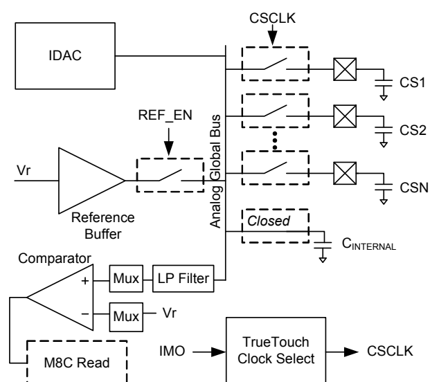
Figure 11-6. Successive Approximation Block Diagram
