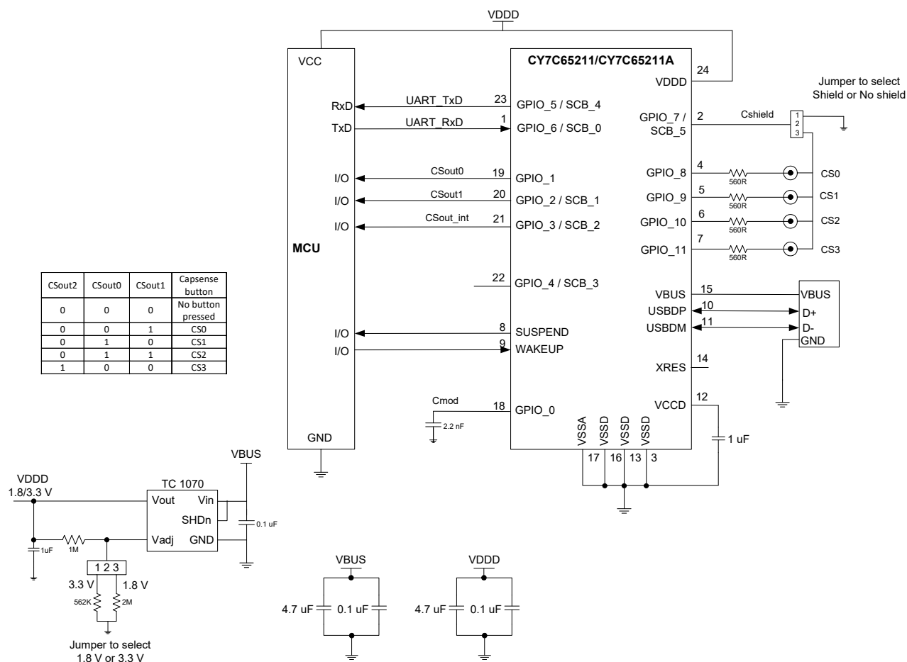
Figure 13. CapSense Schematic
