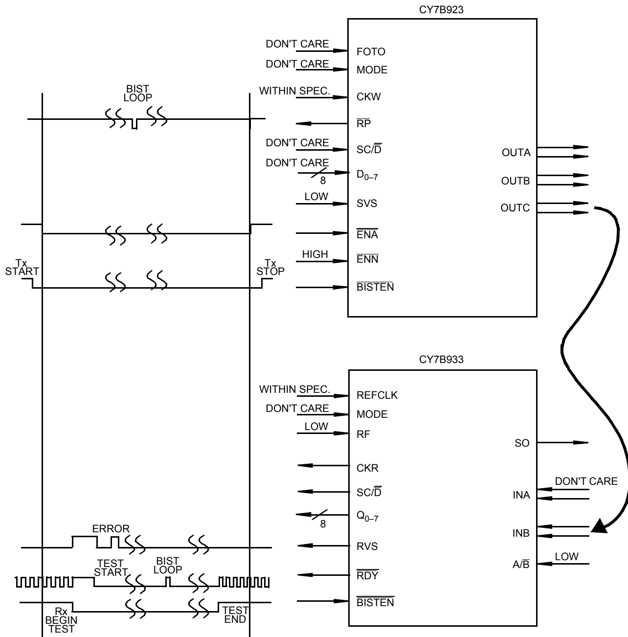
Figure 8. BIST Illustration
